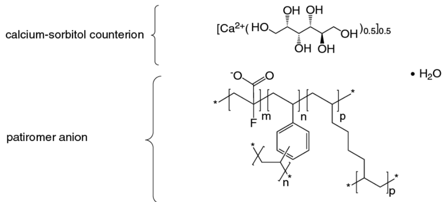
Figure 1: Chemical Structure of Patiromer Sorbitex Calcium
